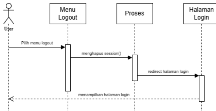
Gambar 1.12 Sequence Diagram Logout
