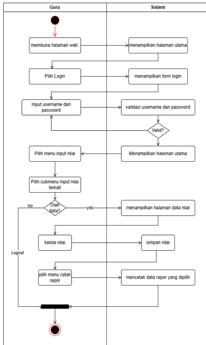
Gambar 1.7 Activity diagram wali kelas
