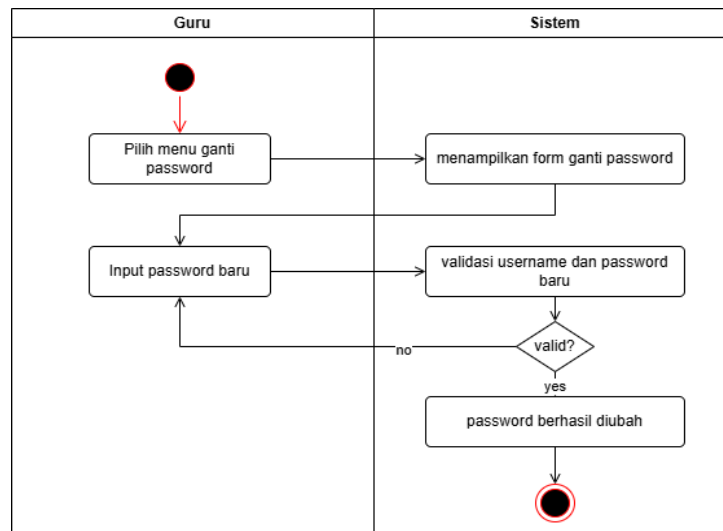
Gambar 1.9 Activity diagram ganti password
