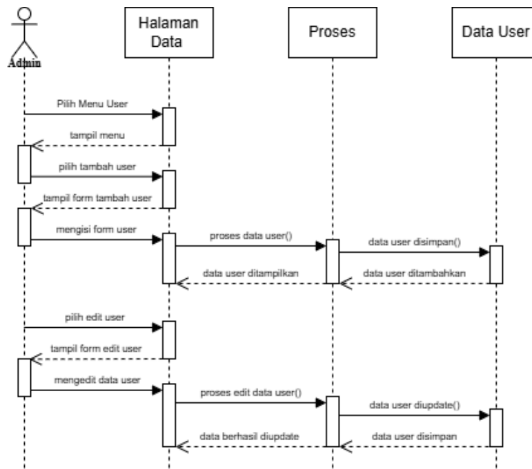
Gambar 1.14 Sequence Diagram Admin Kelola Data User
