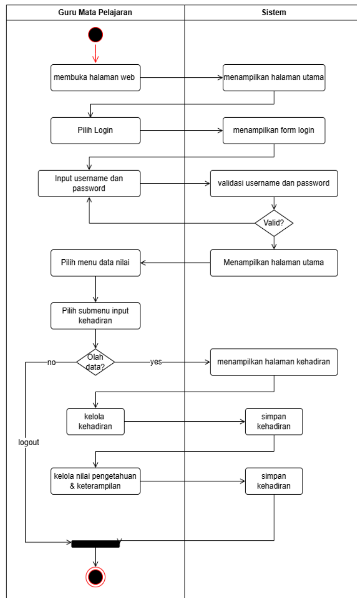
Gambar 1.6 Activity diagram guru mata pelajaran
