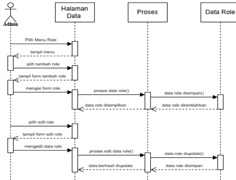
Gambar 1.15 Sequence Diagram Admin Kelola Data Role
