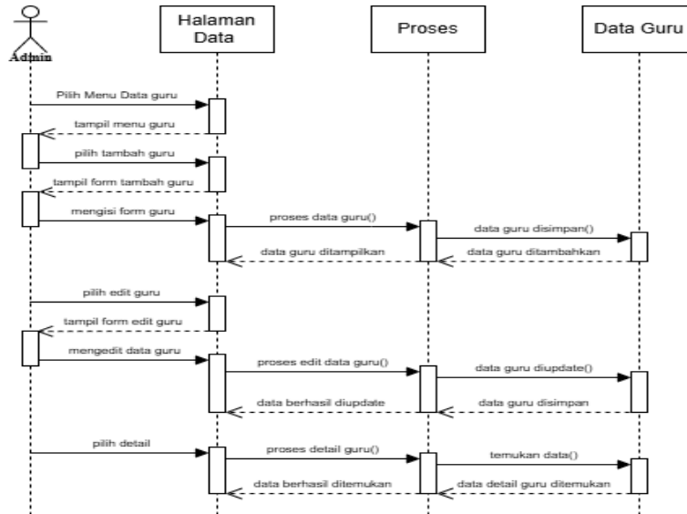
Gambar 1.17 Sequence diagram admin kelola data guru
