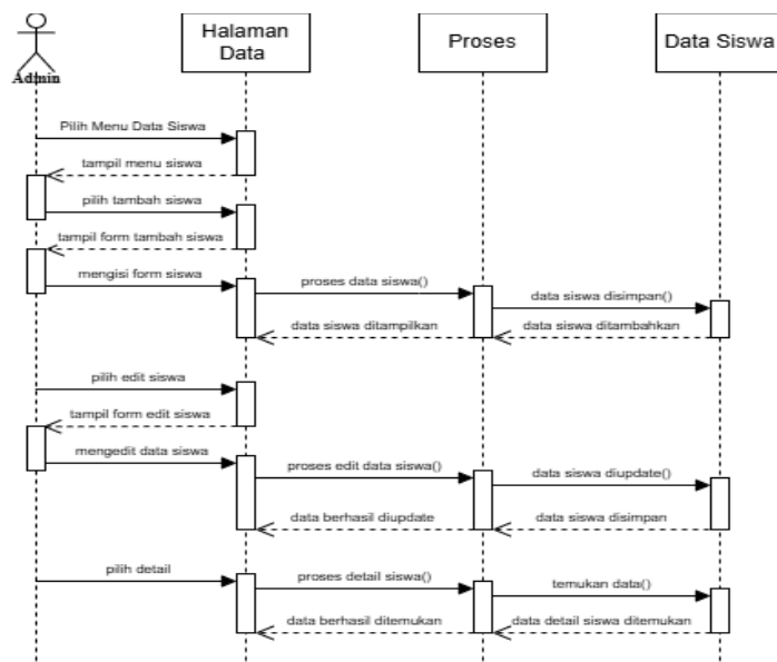
Gambar 1.18 Sequence diagram admin kelola data siswa
