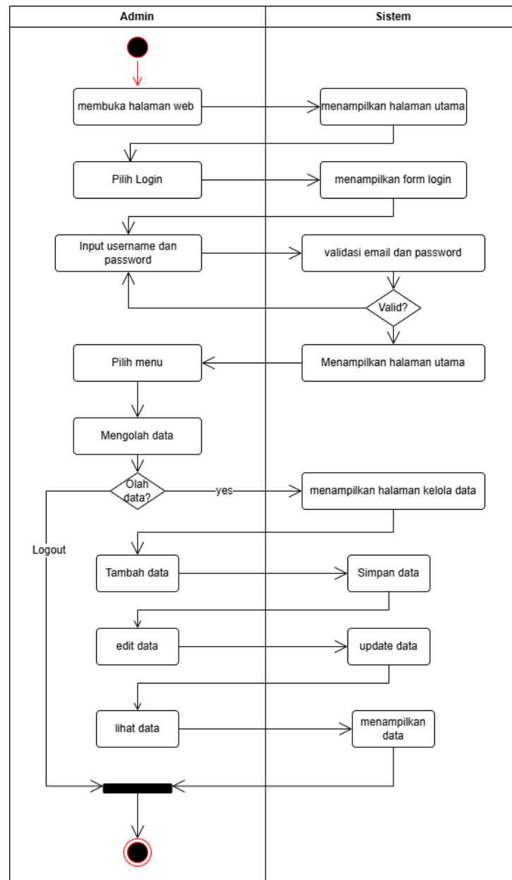
Gambar 1.5 Activity diagram admin
