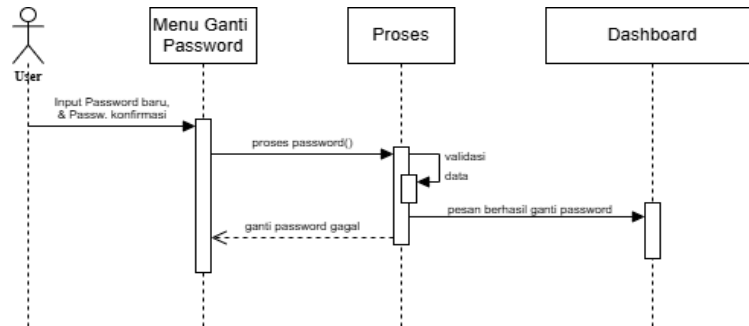
Gambar 1.13 Sequence Diagram Ganti Password
