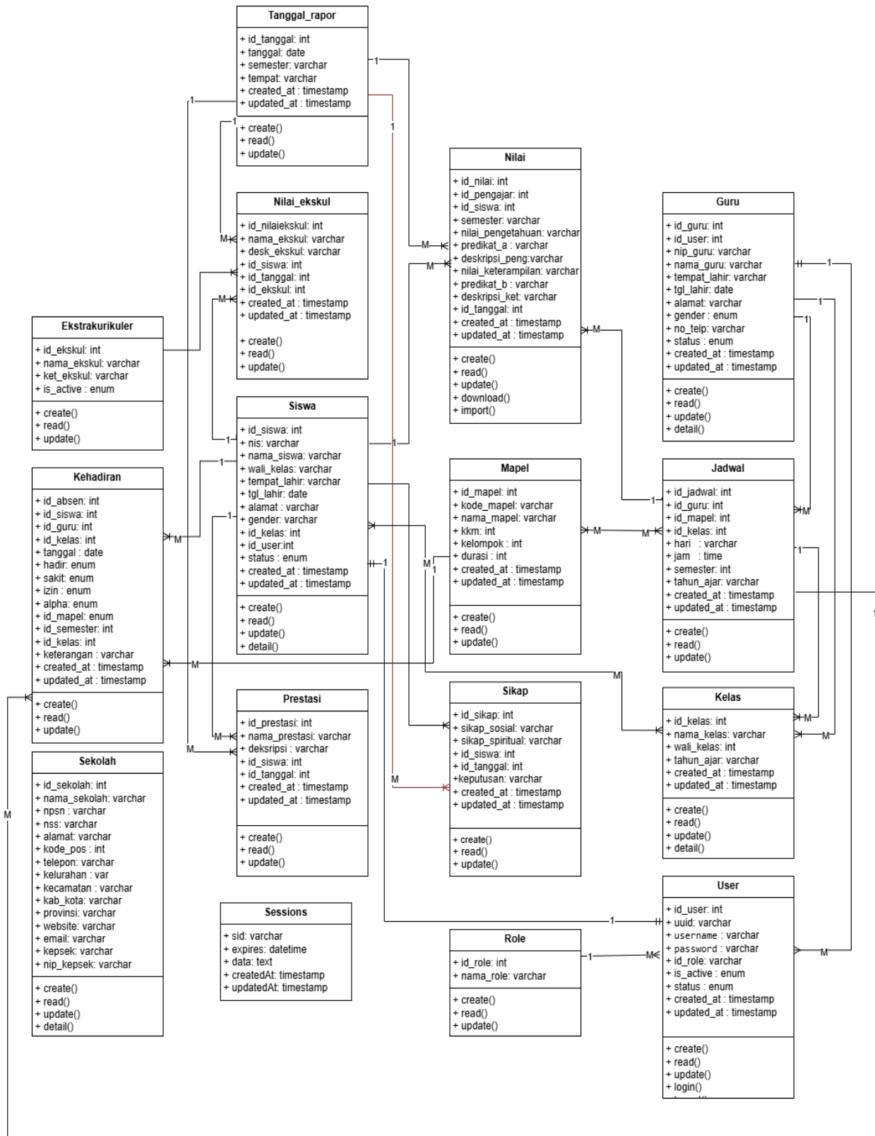
Gambar 1.10 Class Diagram Si E-Raport
