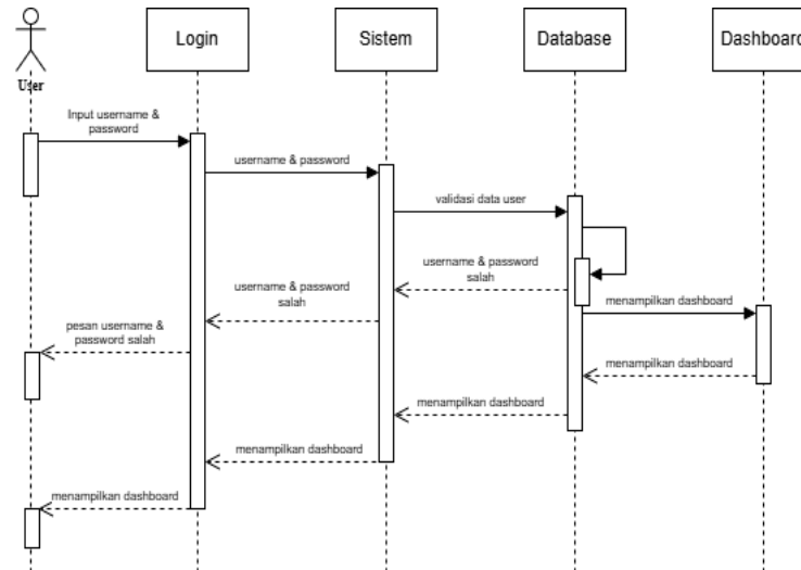
Gambar 1.11 Sequence Diagram Login
