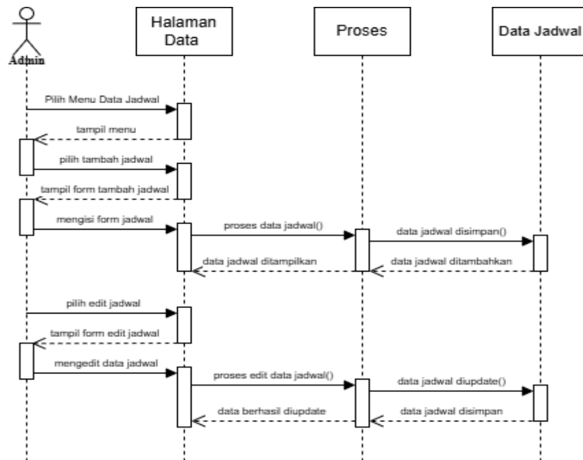
Gambar 1.21 Sequence diagram admin kelola data jadwal
